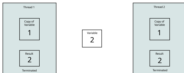
Figure 119: Both Threads Terminated
